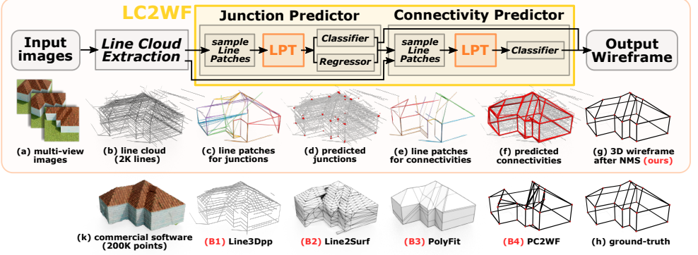
Figure 1: Method Overview. Top: our method takes multi-view images (a) as input and outputs a high-quality 3D wireframe (g). Specifically, we first extract a line cloud (b) from the images, from which we sample line patches (c) and (e) to predict wireframe junctions (d) and connectivities (f) respectively. Bottom: we compare to four baselines: Line3Dpp [17] (B1) produces abstracted line clouds from the input noisy line clouds (b). Line2Surf [60] (B2) takes (B1) as input and outputs a triangle mesh. From the point cloud (k), PolyFit [69] (B3) produces a polygonal mesh, while PC2WF [67] (B4) outputs a 3D wireframe.
