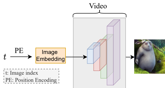
(a) NeRV with position embedding (PE)
