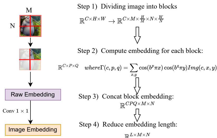
(c) CNeRV encoder: Content-adaptive Encoding
